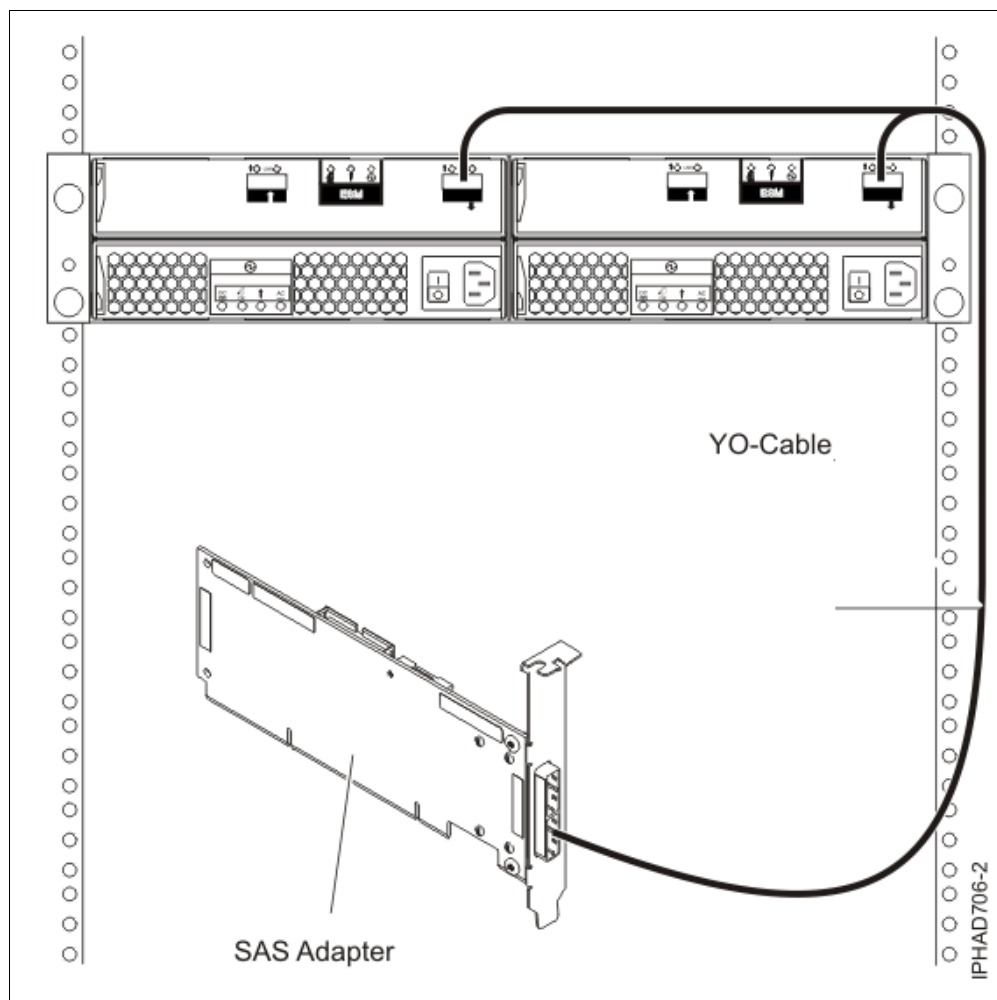
Figure 6-4 5886 to a system unit connection example using a YO cable
