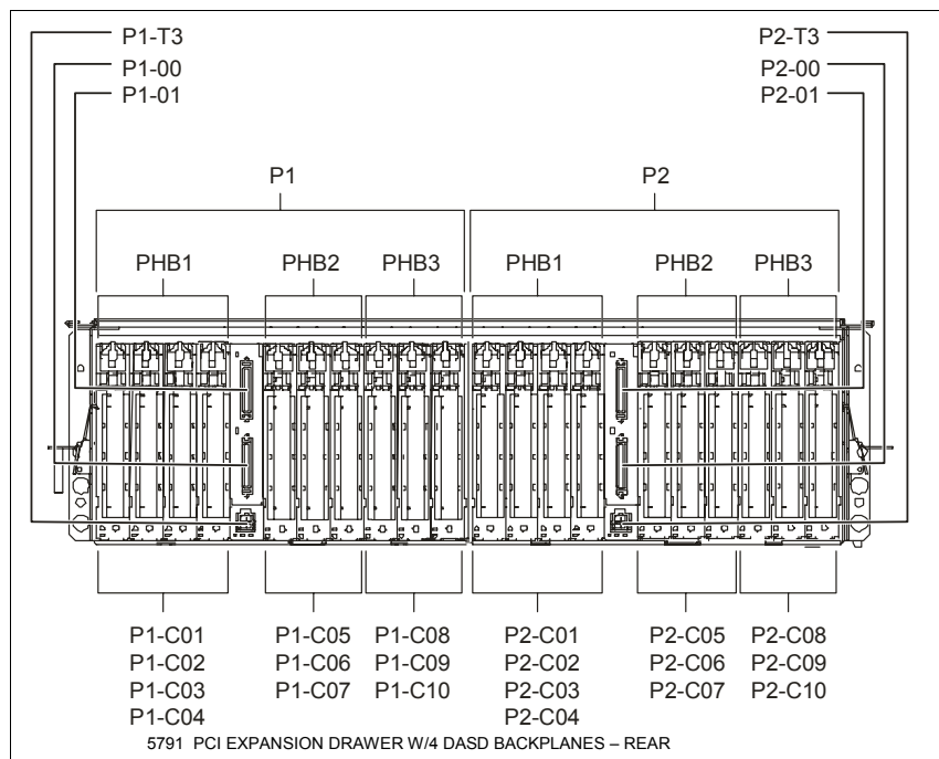
Figure 9-14 Back view of #5791
