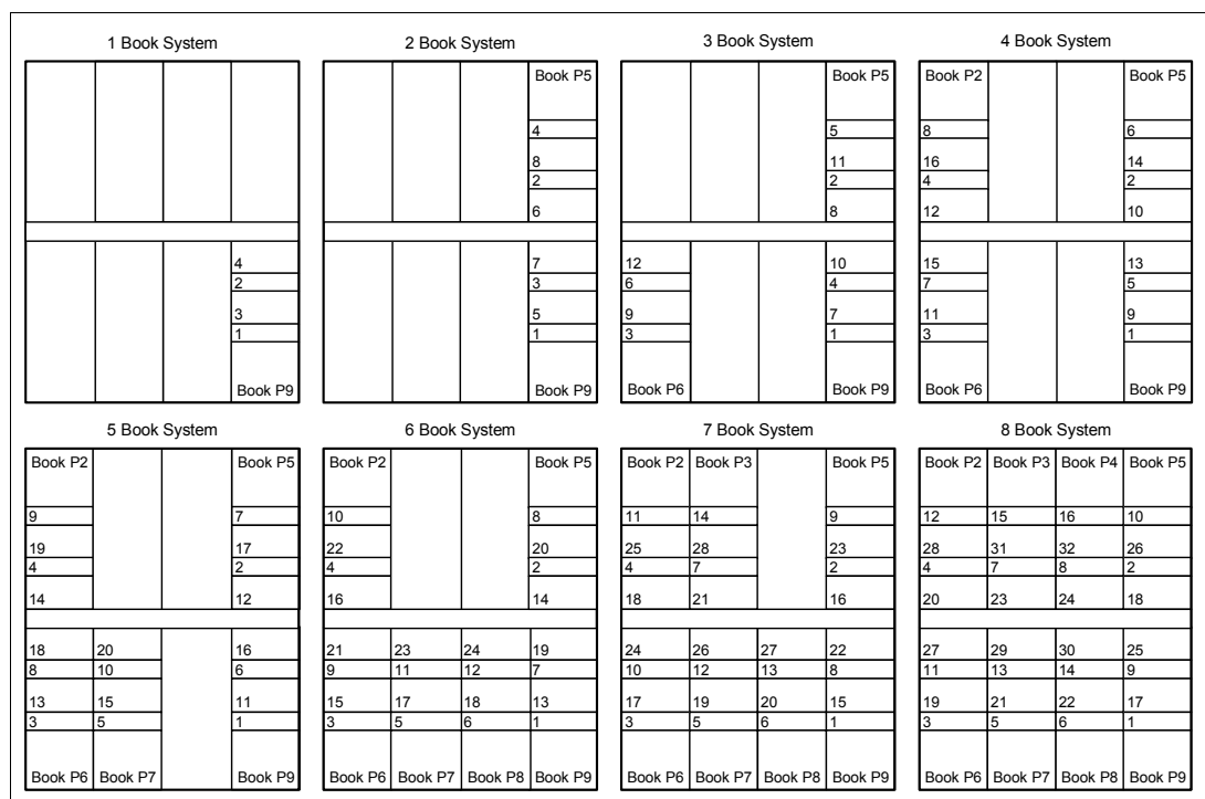
Figure 3-26 One through eight processor books (nodes) view of I/O Hub (GX adapter) plugging rules
