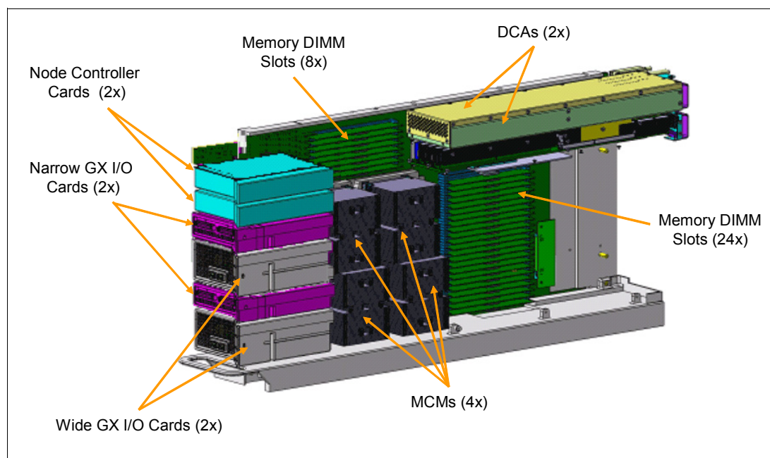
Figure 3-19 DDR2 buffered memory
