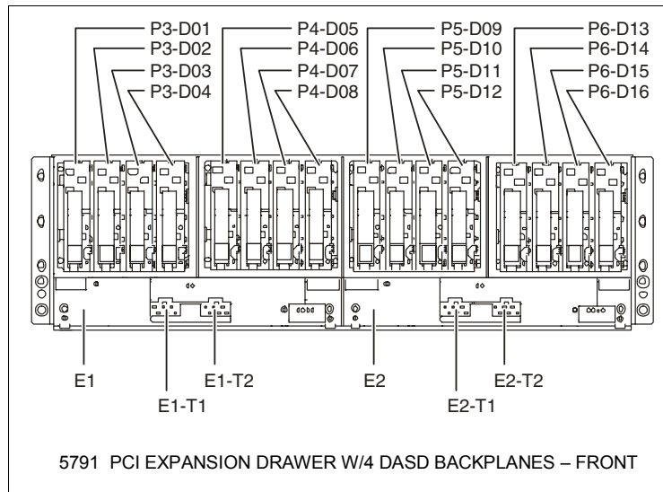
Figure 9-13 Front view of #5791
