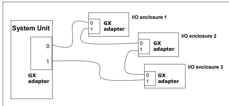
Figure 9-26 Placement of RIO-2 I/O enclosures on the same loop
