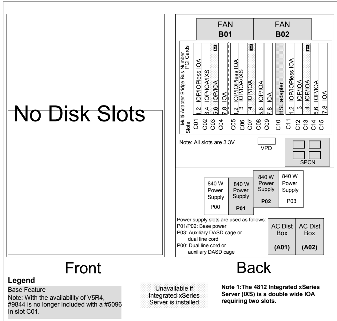
Figure 9-4 #5096 PCI-X expansion tower (no disk)
