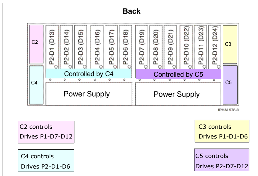
Figure 5-2 Back view of the #5786 TotalStorage Expansion 24 Disk Drawer
