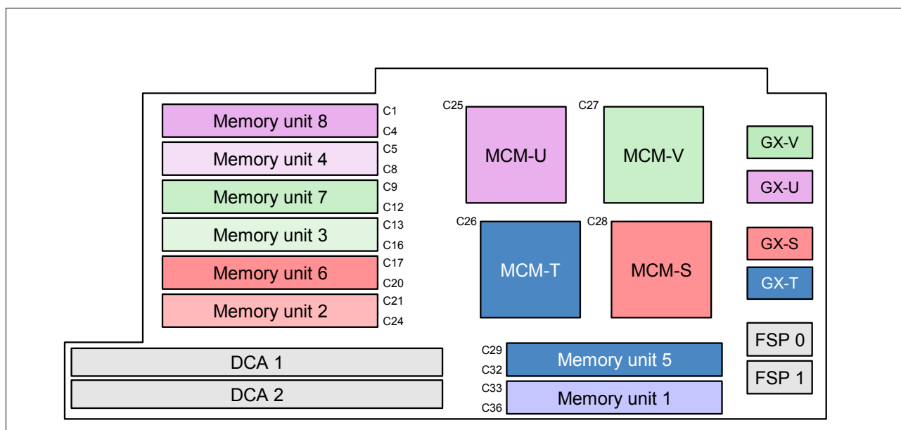
Figure 3-20 Processor book with MCM and memory locations
