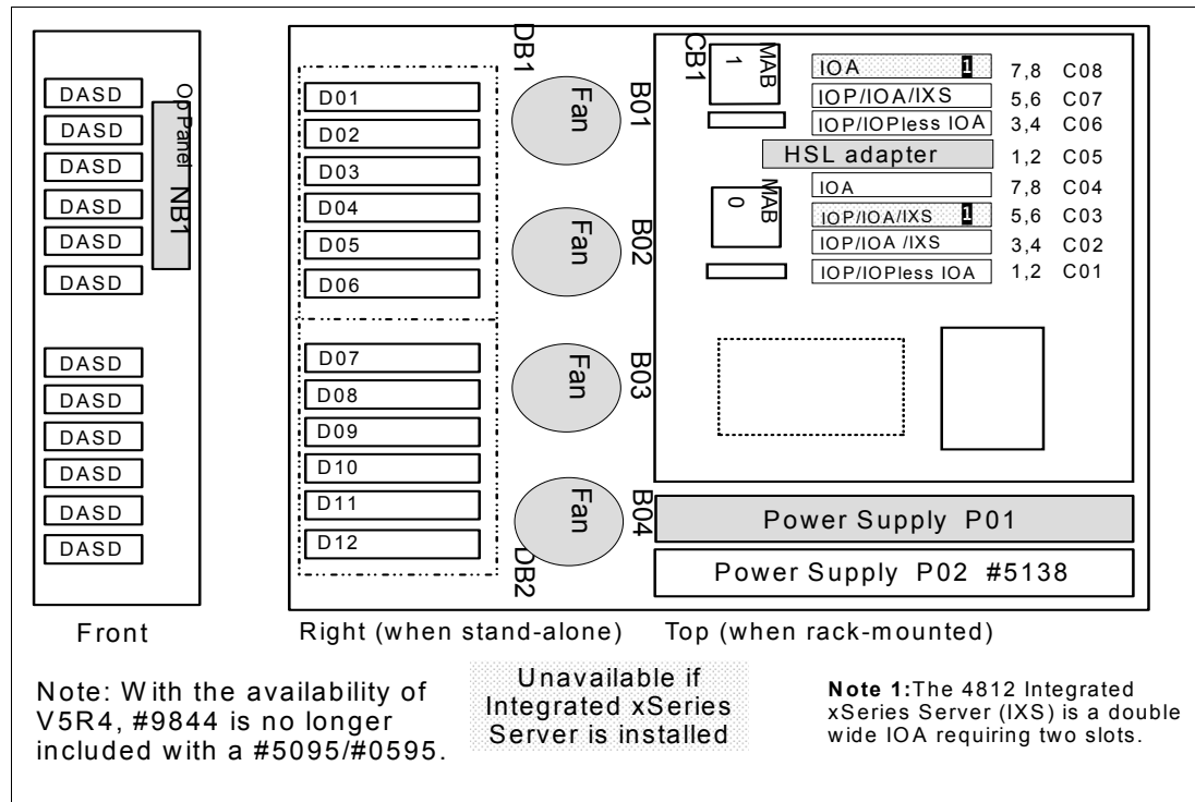
Figure 9-3 #5095/#0595 PCI-X Expansion Tower
