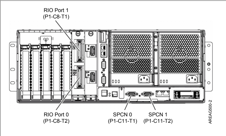
Figure 2-14 9117-MMA RIO-2 and SPCN connector locations
