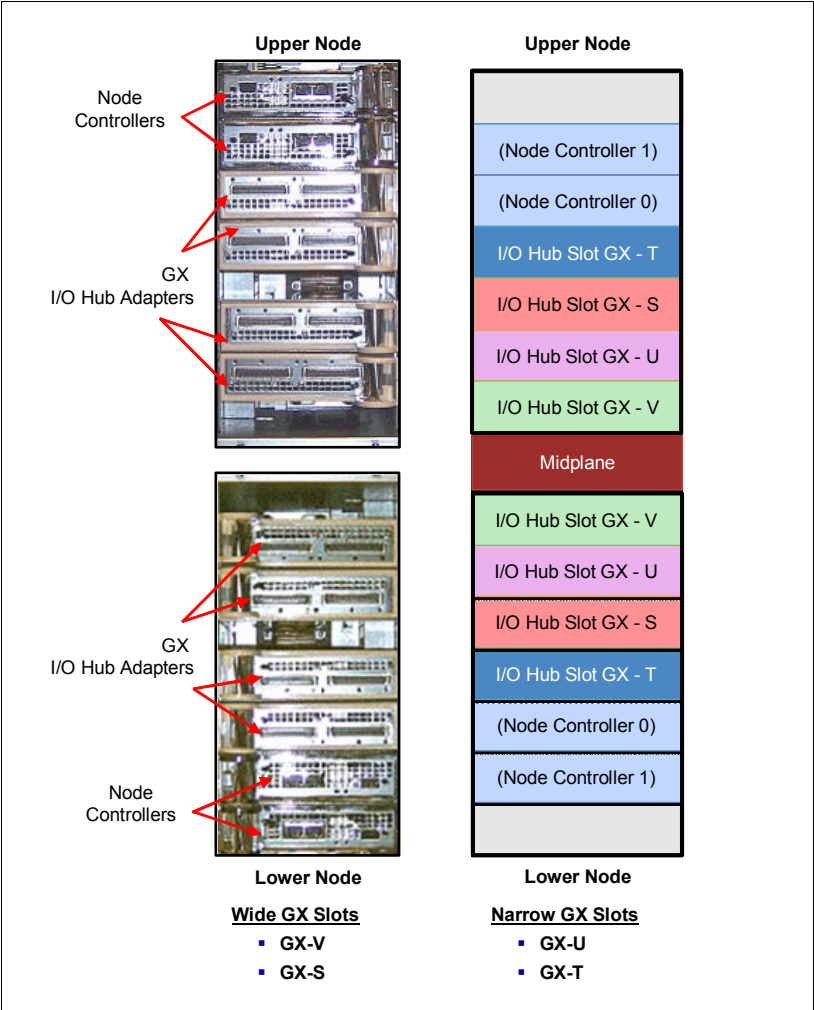
Figure 3-21 GX adapter placement
