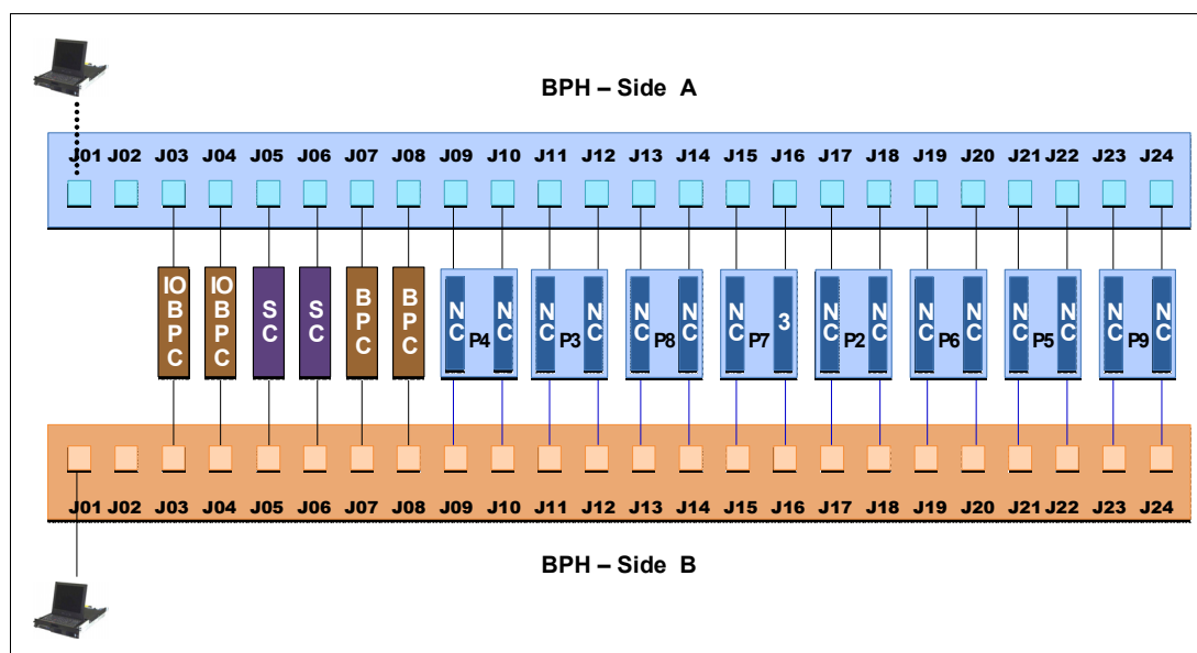
Figure 3-13 Bulk power hubs
