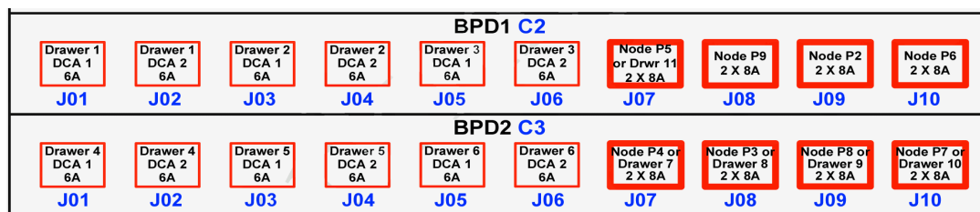
Figure 3-15 Bulk power distribution assembly
