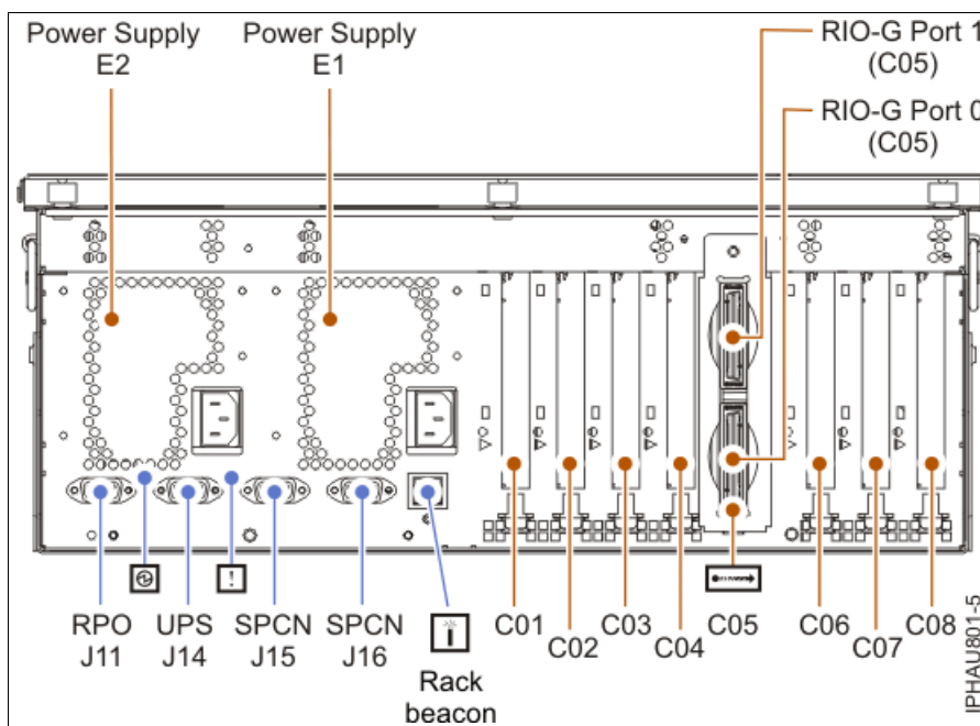
Figure 9-24 7311-D20 rear view
