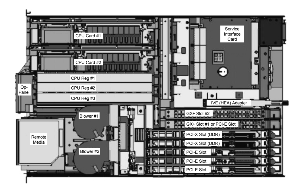
Figure 2-20 9117-MMA top view
