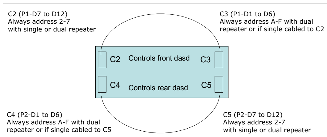
Figure 5-3 Card slot device addressing rules using #5741 single and #5742 dual repeaters
