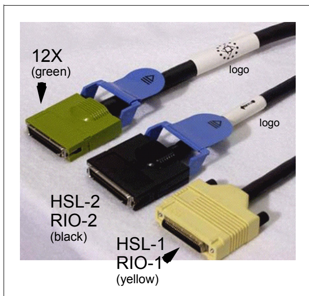
Figure 11-1 12X, HSL-2/RIO-2, HSL-1/RIO-1 cables
