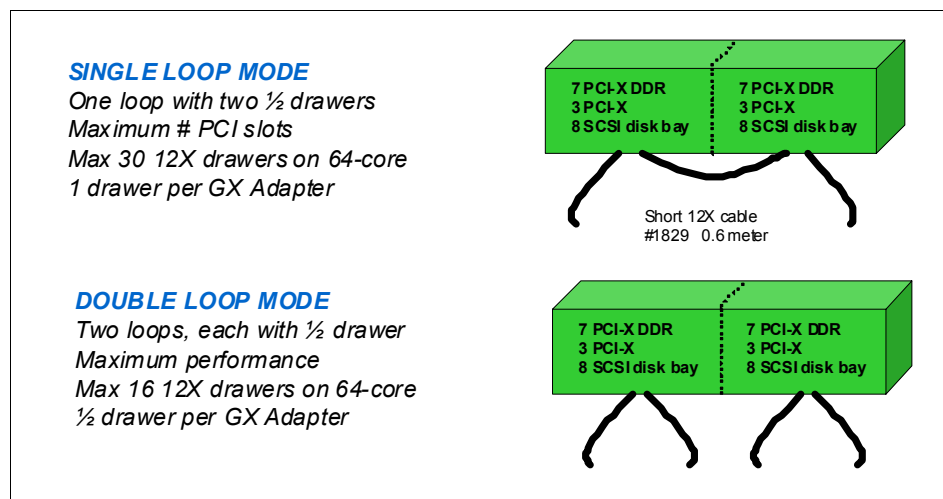
Figure 4-1 IBM #5797, #5798 loop connection options
