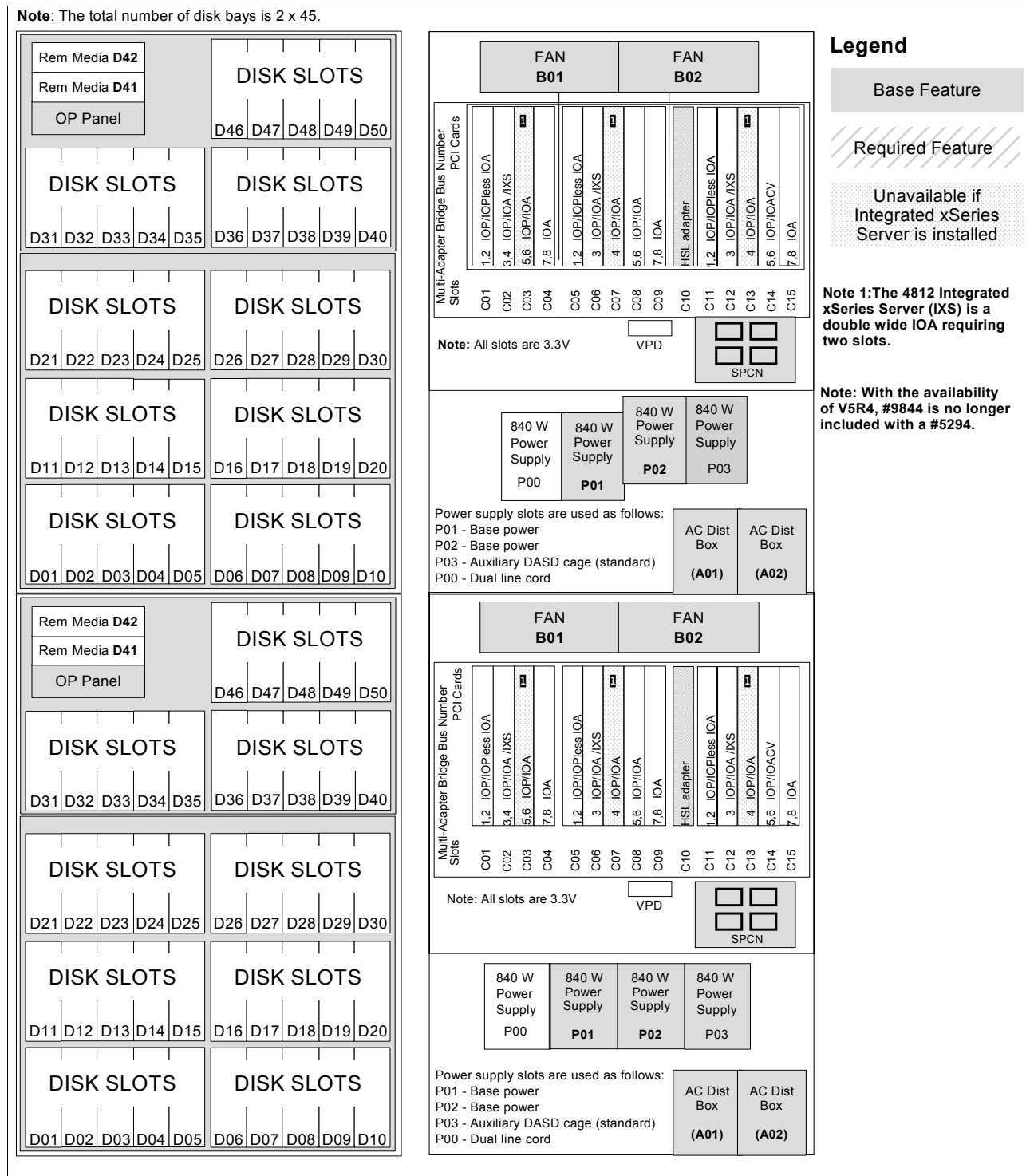
Figure 9-5 #5294 1.8 m I/O expansion tower
