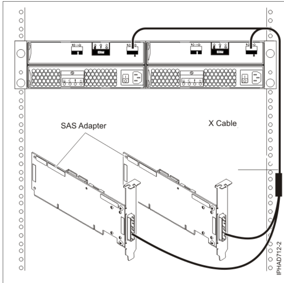
Figure 6-6 HA one and two system RAID
