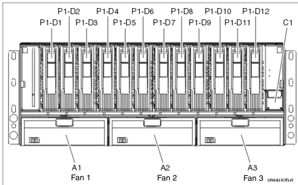
Figure 9-8 Front view of the #5786
