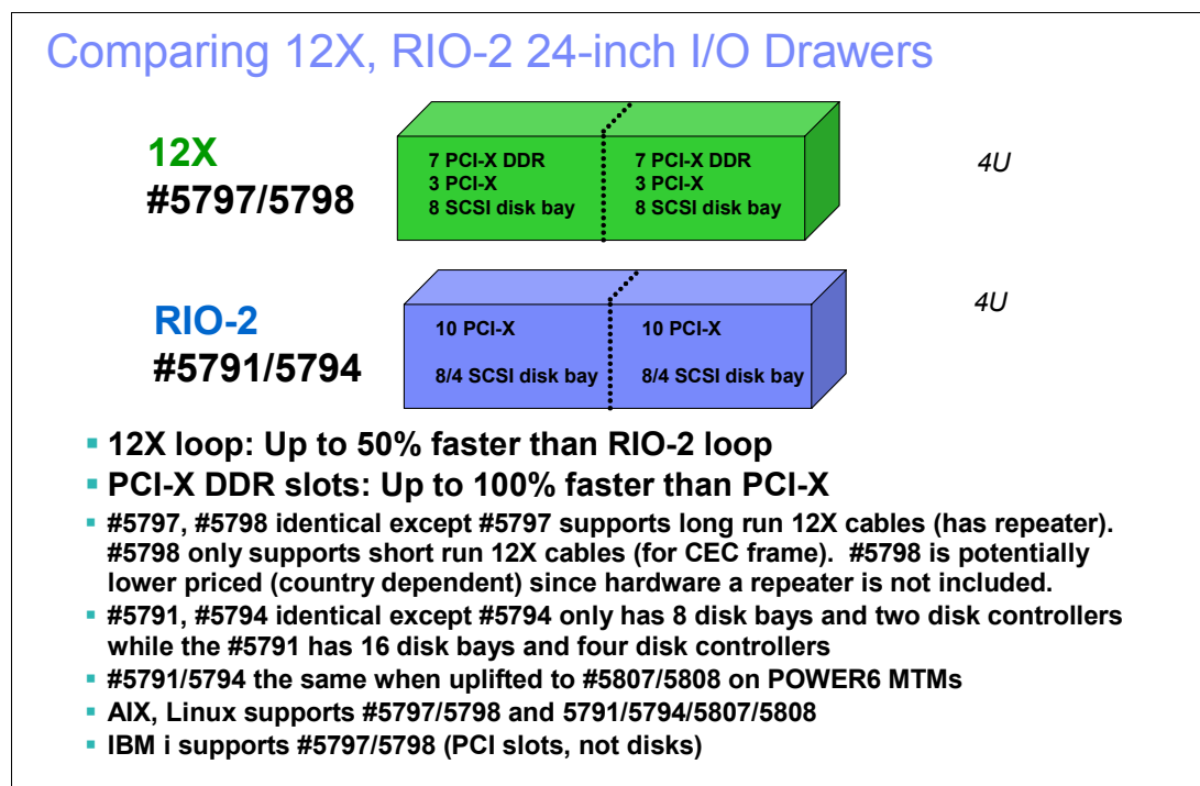
Figure 4-2 Comparison of RIO-2 and 12X using #5797, #5798 I/O drawers
