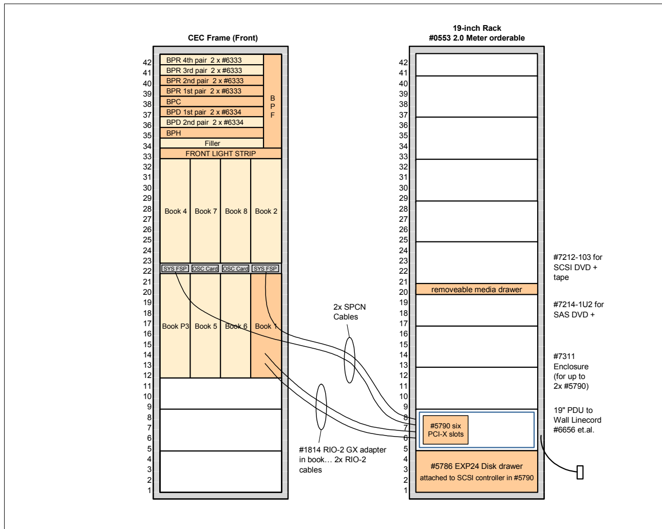
Figure 3-33 Example 595 system (CEC) frame with only a 19 inch rack containing I/O enclosure used by IBM i
