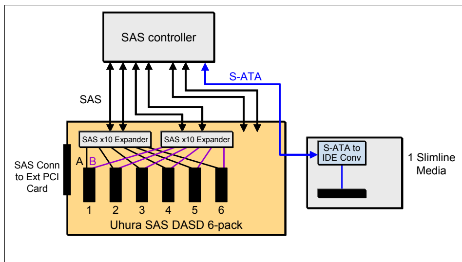
Figure 4-3 SAS disk controller and DVD connection
