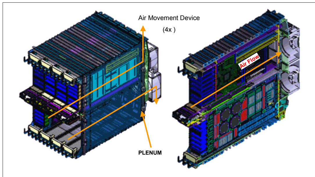
Figure 3-18 CEC internal air flow
