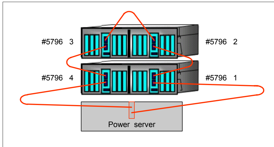
Figure 11-2 Cabling example of two SAS enclosures to a POWER6 system
