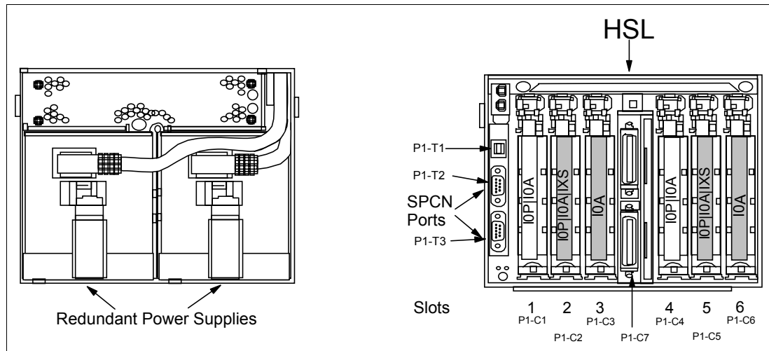
Figure 9-10 #5790 PCI Expansion Drawer
