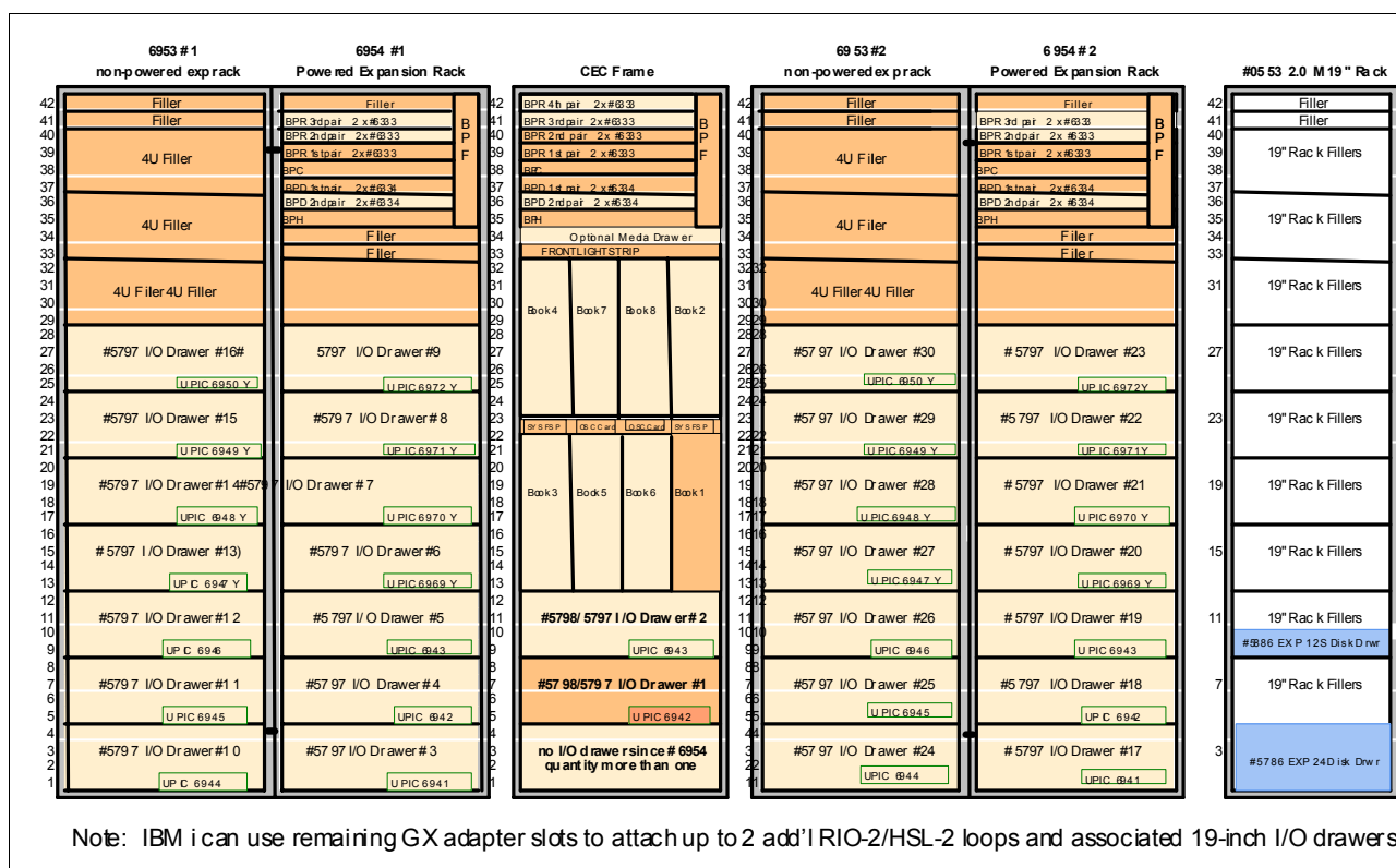
Figure 3-30 9119-FHA I/O expansion drawer locations
